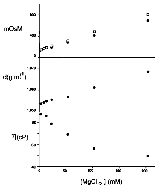
FIGURE 8 The osmolality, density, and viscosity of a solution of 10% dextran sulphate to which increasing concentrations of \text{MgCl}_2 were added. \square , observed osmolality; \bullet , osmolality calculated assuming that the contributions of \text{MgCl}_2 and dextran sulphate were additive.
