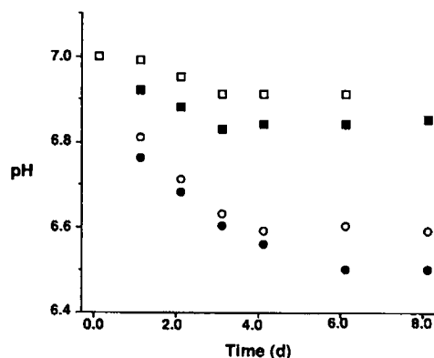
FIGURE 4 The change in pH of buffer solutions equilibrated with Biogel P-4 #321374. The solutions were all initially 10 mM and pH 7. □, Tris; ■, histidine; ○, \text{KP}_i ; ●, \text{NaP}_i .
