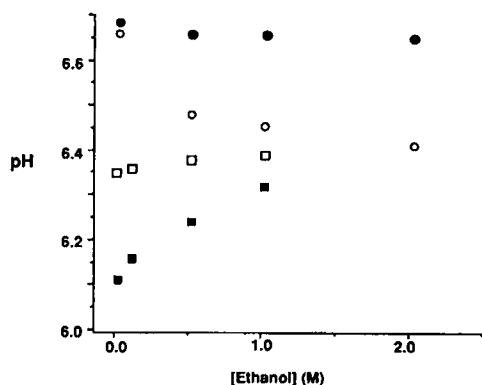
FIGURE 2 The effects of increasing concentrations of ethanol in either 10 mM \text{NaP}_i or 10 mM \text{KP}_i , pH 7, on the pH of a solution external to Biogel 4. \text{NaP}_i ; ■, #307192-00; ●, #321374; \text{KP}_i ; □, #307192-00; ○, #321374. Conditions were the same as in Fig. 1.
