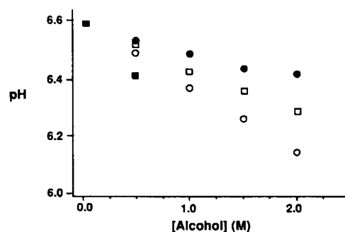
FIGURE 3 The effects of increasing concentrations of alcohols on the pH of a solution of 10 mM \text{KP}_i , pH 7, equilibrated with Biogel P-4 #321374. ●, methanol; □, ethanol; ○, propanol; ■, butanol.
