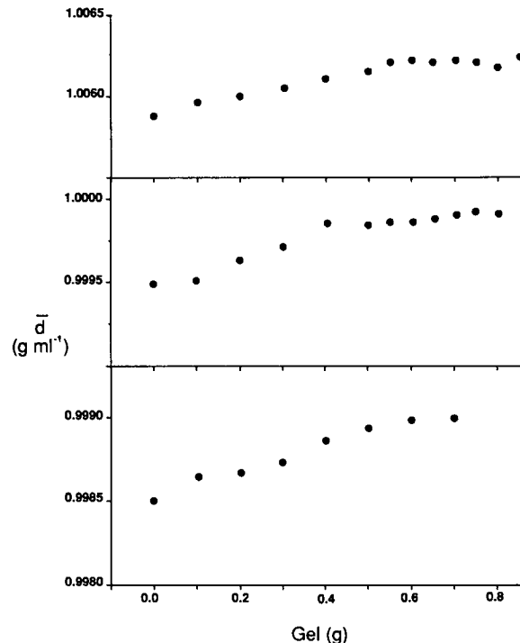
FIGURE 7 The average density of solutions of MgCl 2 equilibrated in density bottles with increasing weights of Biogel P-4 #307192-00. Top, 100 mM; middle, 20 mM; bottom, 5 mM.
