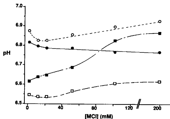
FIGURE 1 The effect of increasing concentrations of NaCl or KCl on the pH of a solution external to Biogel P-4. NaCl added to 10 mM \text{NaPi} , pH 7: ■, #307192-00; ●, #321374; KCl added to 10 mM \text{KPi} , pH 7: □, #307192-00; ○, #321374. 0.4 gel was equilibrated with 2.8 ml (#307192-00) or 2.4 ml (#321374) of solution. Each point is the mean of duplicates with standard deviation smaller than the symbol.
